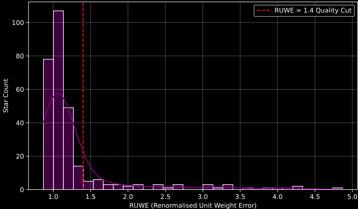
GALAH DR4 Field [193] RUWE Distribution (n= 291)
