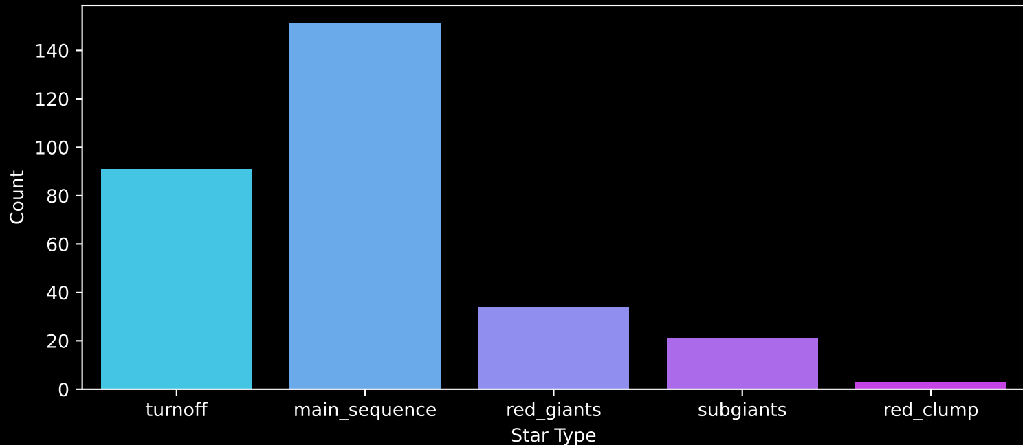
GALAH DR4 Field: [193] Count plot of Star Type
