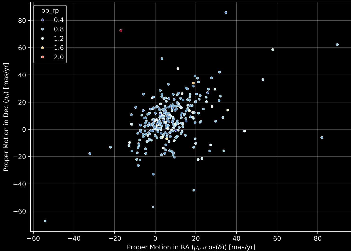
GALAH DR4 Field: [193] Proper Motion Diagram (n= 300)
